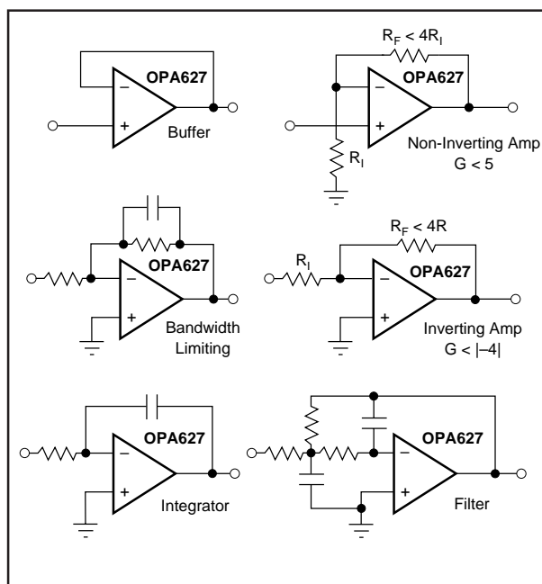
FIGURE 1. Circuits with Noise Gain Less than Five Require the OPA627 for Proper Stability.
