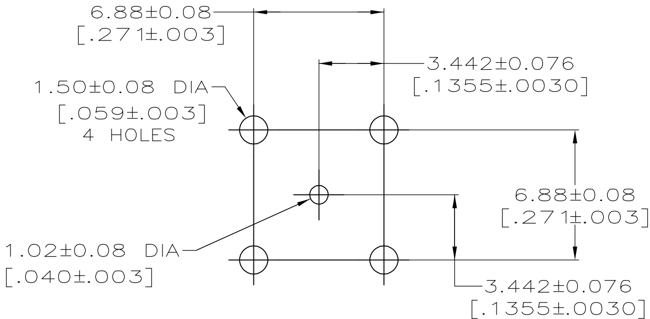
PCB CONFIGURATION
