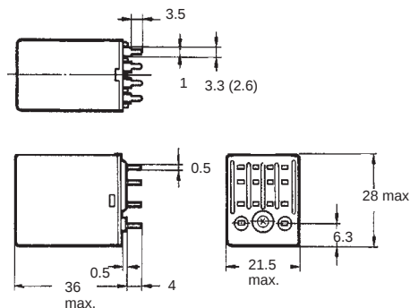
MY4-02 (4PDT)
