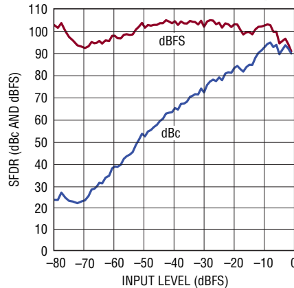
LTC2171-12: SFDR vs Input Level, f_{IN} = 70\text{MHz} , 2\text{V} Range, 40\text{MSPS}
