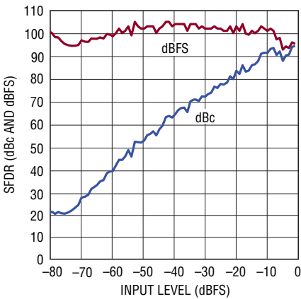
LTC2170-12: SFDR vs Input Level, f_{IN} = 70\text{MHz} , 2V Range, 25Msps
