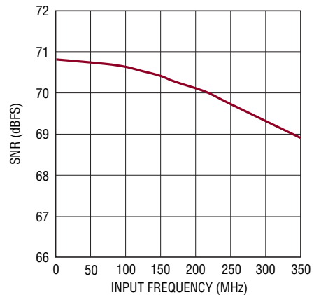
LTC2171-12: SNR vs Input Frequency, -1\text{dBFS} , 2\text{V} Range, 40\text{MSPS}
