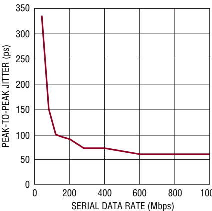
DCO Cycle-Cycle Jitter vs Serial Data Rate
