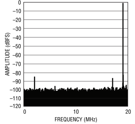
LTC2171-12: 8k Point FFT, f_{IN} = 139\text{MHz} , -1\text{dBFS} , 40\text{MSPS}
