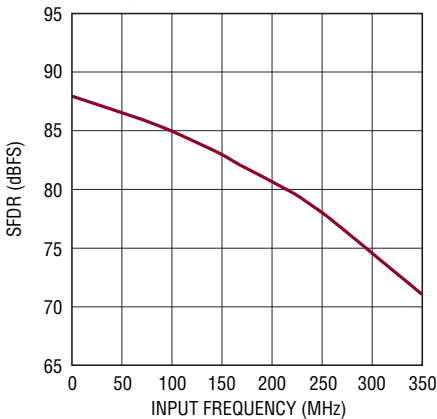
LTC2171-12: SFDR vs Input Frequency, -1\text{dBFS} , 2\text{V} Range, 40\text{MSPS}
