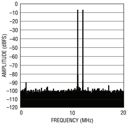
LTC2171-12: 8k Point 2-Tone FFT, f_{IN} = 68\text{MHz} , 69\text{MHz} , -1\text{dBFS} , 40\text{MSPS}
