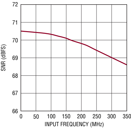
LTC2170-12: SNR vs Input Frequency, -1dBFS, 2V Range, 25Msps
