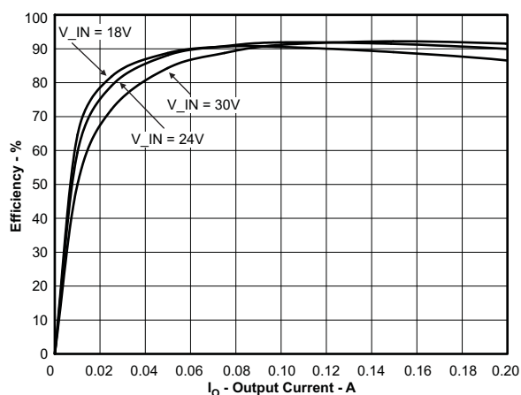
Figure 1. TPS54060EVM-590 Efficiency
