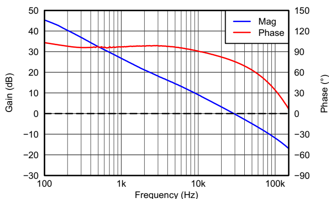
Figure 2-5. TPS54020EVM-082 Loop Bode Response
