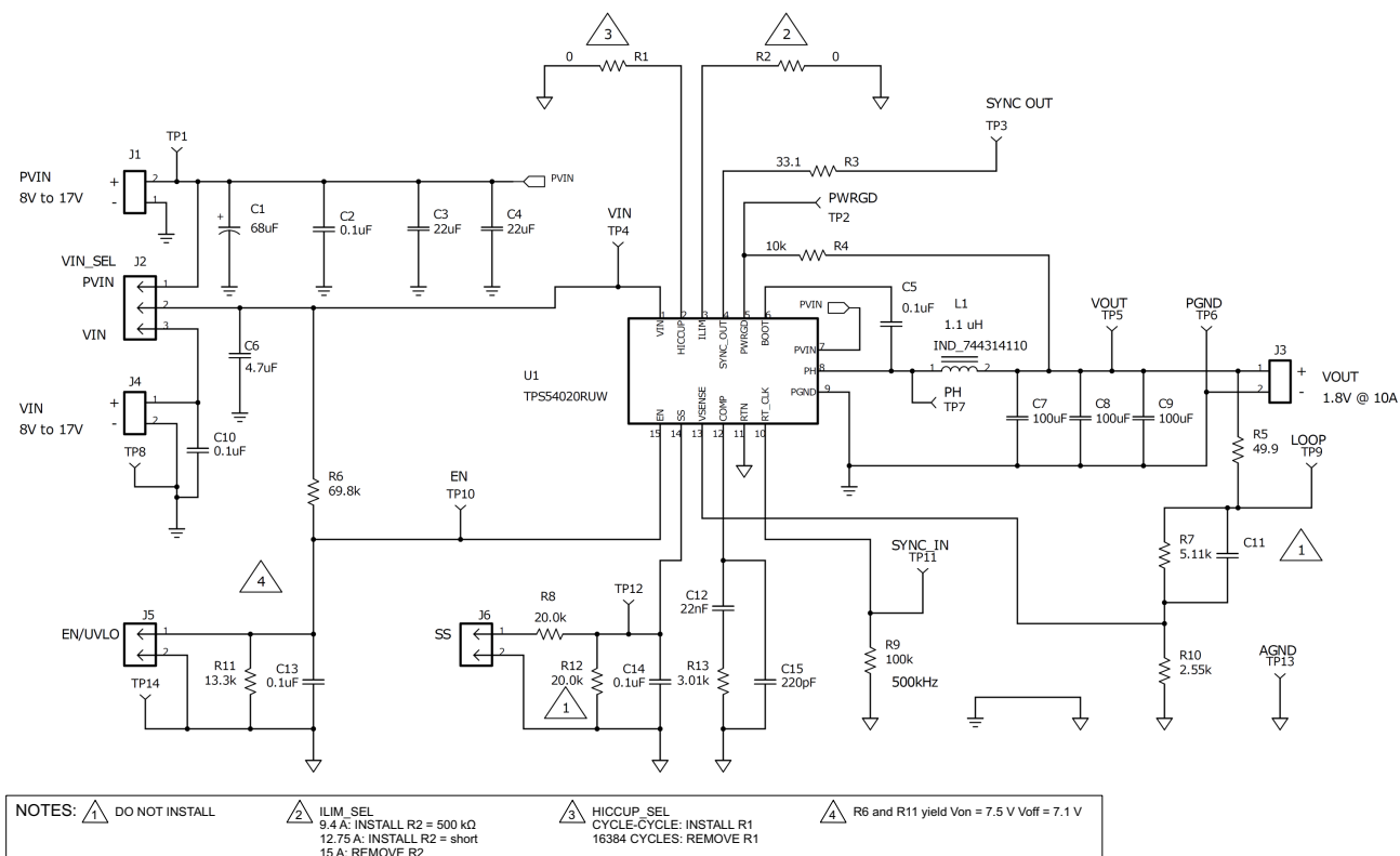
Figure 4-1. TPS54020EVM-082 Schematic
