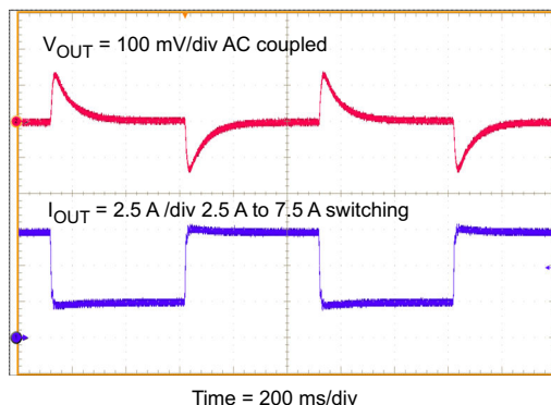
Figure 2-4. TPS54020EVM-082 Transient Response
