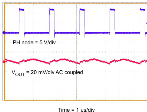
Figure 2-6. TPS54020EVM-082 Output Ripple
