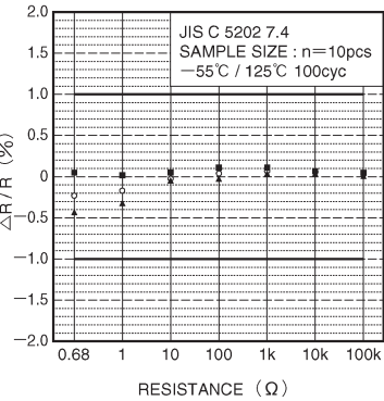
Fig.17 Temperature cycling
