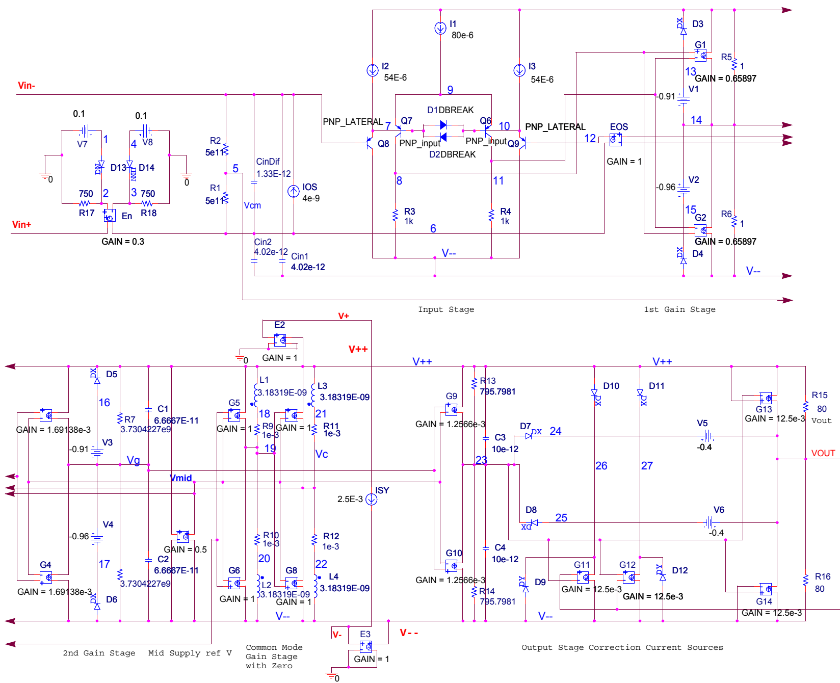
FIGURE 64. SPICE SCHEMATIC
