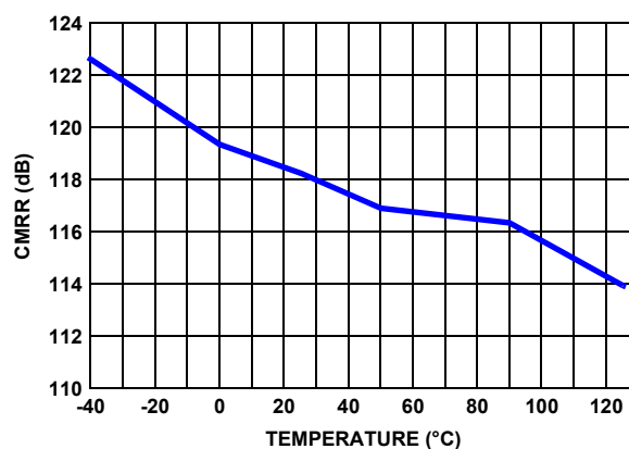
FIGURE 16. ISL28118 CMRR vs TEMPERATURE, V_S = \pm 5V
