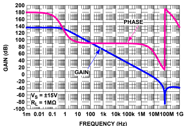
FIGURE 69. SIMULATED OPEN-LOOP GAIN, PHASE vs FREQUENCY
