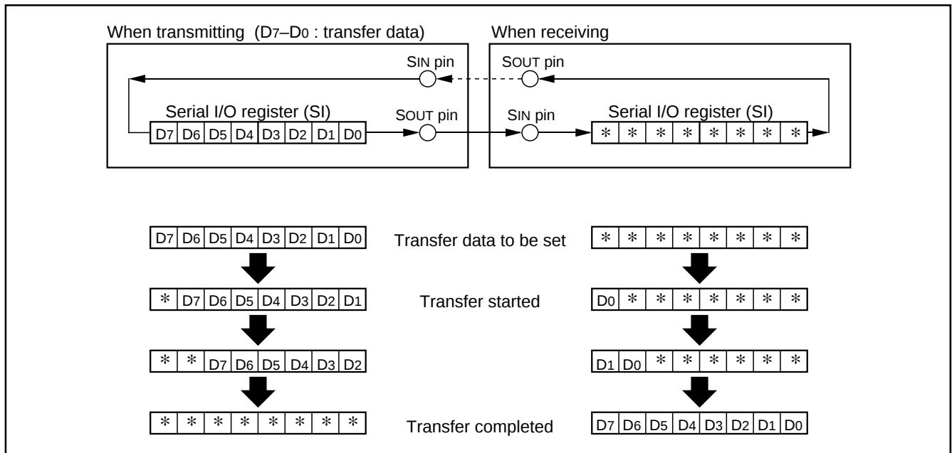
Fig. 23 Serial I/O register state when transferring
