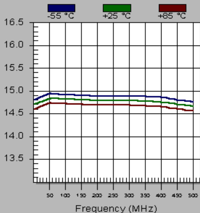
TM6520 Gain (dB)
