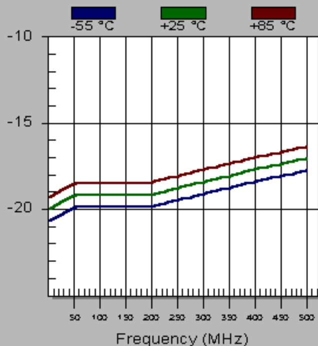
TM6520 Reverse Isolation (dB)
