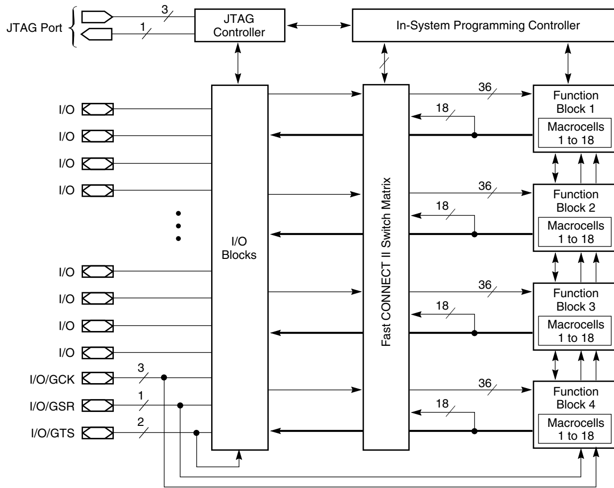
Figure 2: XC9572 Architecture
