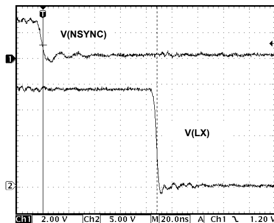
FIGURE 15. NSYNC TO LX SYNCHRONIZATION DELAY
