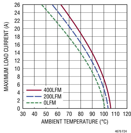
Figure 24. 12V to 1.8V Derating Curve, with Heat Sink
