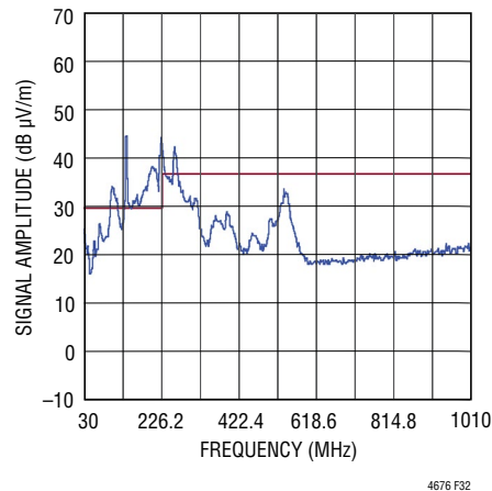
Figure 32. Radiated Emissions Scan of LTM4676 Producing 1V OUT at 26A, from 12V IN . DC1811 Hardware with Outputs Paralleled. No Snubbers Applied. f_{SW} = 350kHz. Measured in a 10m Chamber. Peak Detect Method
