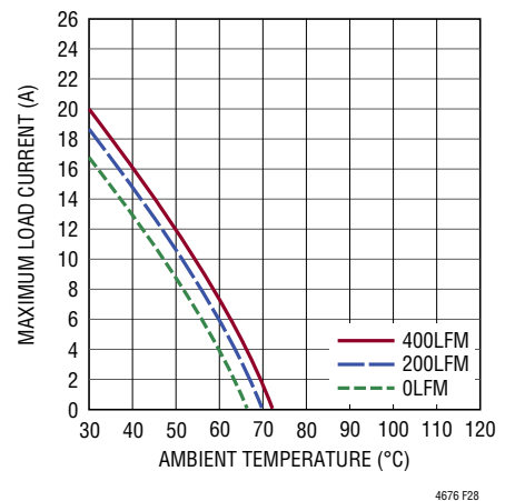
Figure 28. 24V to 3.3V Derating Curve, with Heat Sink
