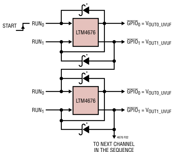
Voltage Based Sequencing by Cascading \overline{\text{GPIO}}_n Pins Into \text{RUN}_n Pins ( \text{MFR\_GPIO\_PROPAGATE} = \text{XXX1X00XX00XXXXX}_b and \text{MFR\_GPIO\_RESPONSE} = 0x00 )
