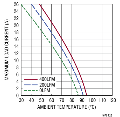
Figure 25. 24V to 1.8V Derating Curve, with Heat Sink
