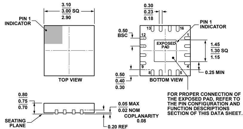
Figure 68. 16-Lead Lead Frame Chip Scale Package [LFCSP_WQ] 3 mm x 3 mm Body, Very Very Thin Quad (CP-16-21) Dimensions shown in millimeters
