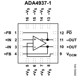
Figure 1. ADA4937-1
