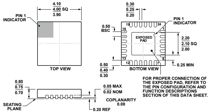
Figure 69. 24-Lead Lead Frame Chip Scale Package [LFCSP_WQ] 4 mm x 4 mm Body, Very Very Thin Quad (CP-24-10) Dimensions shown in millimeters
