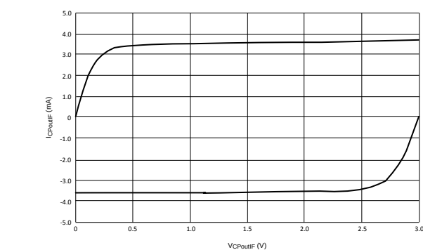
Figure 16. IF PLL Charge Pump Current
