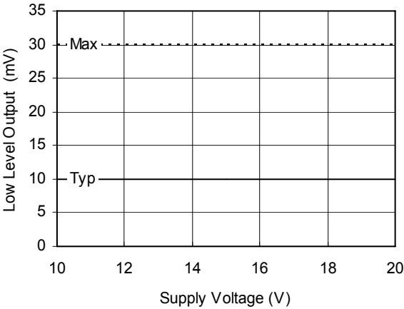
Figure 10B. Low Level Output vs. Supply Voltage ( I_o = 2\text{mA} )
