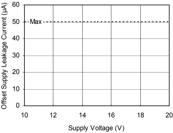
Figure 11B. Offset Supply Leakage Current vs. Supply Voltage
