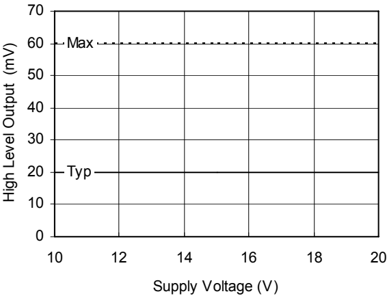
Figure 9B. High Level Output vs. Supply Voltage ( I_o = 2\text{mA} )
