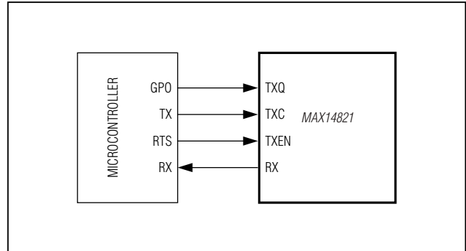
Figure 13. UART Interface
