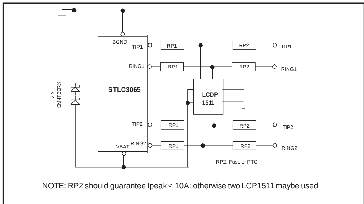
Figure B2. Standard overloltage protection configuration for k20 compliance
