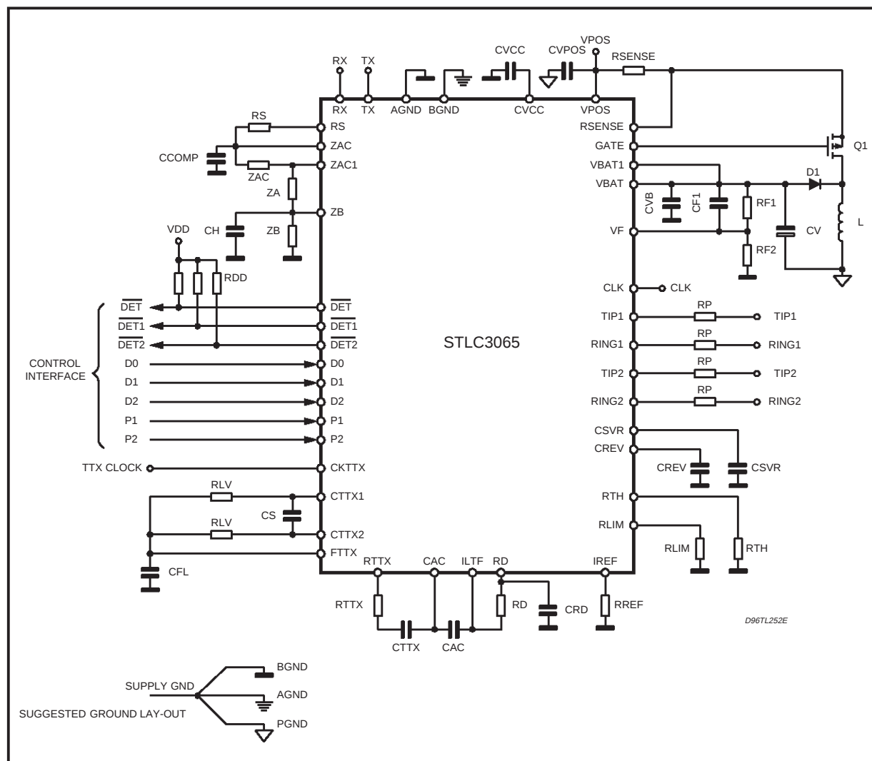
Figure 8. Application diagram.
