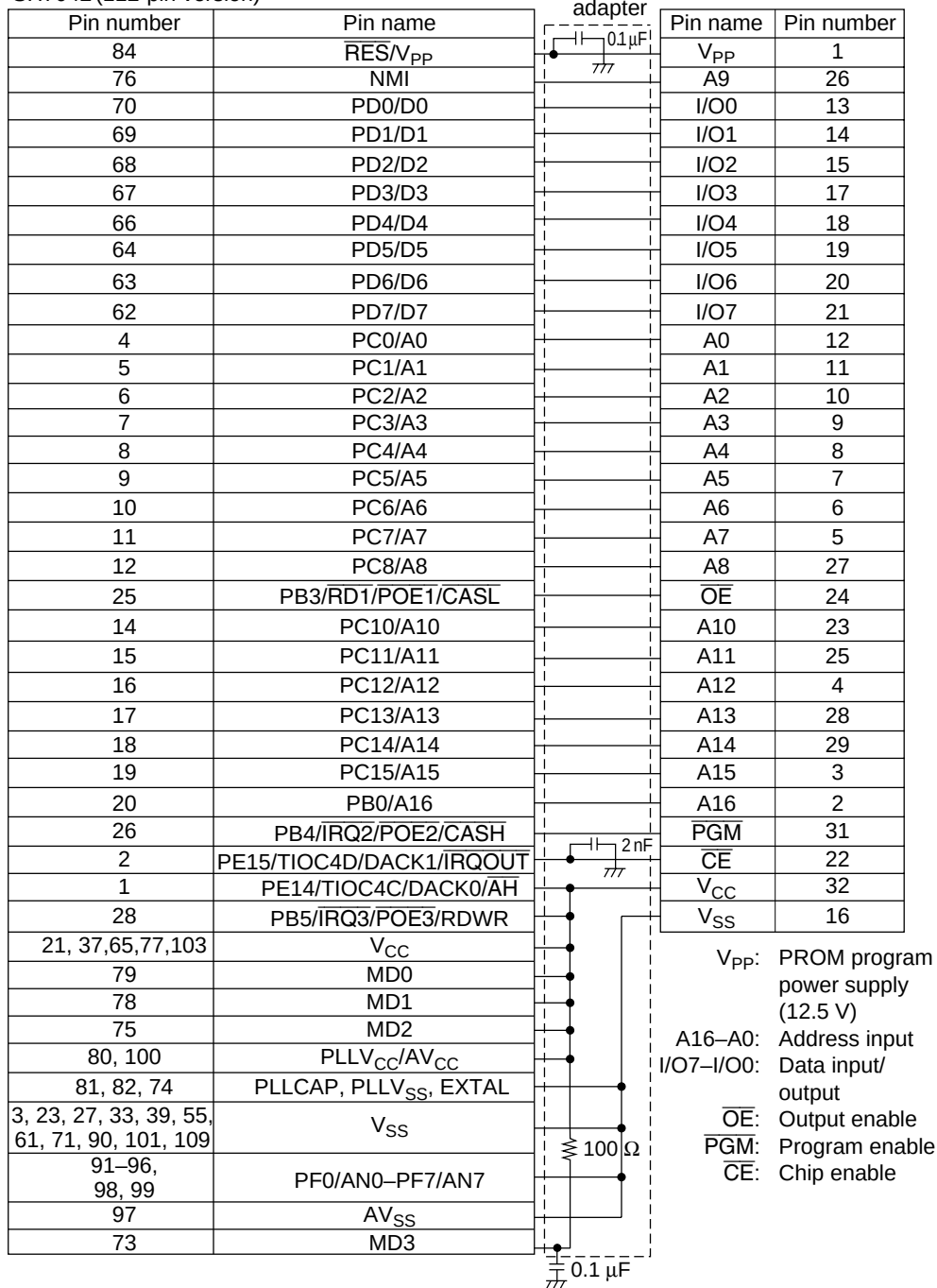
SH7042 (112-pin version)
