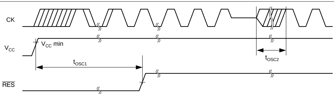
Figure 25.3 Oscillation Settling Time
