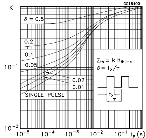
Figure 3: Thermal impedance
