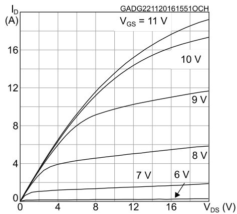
Figure 4: Output characteristics
