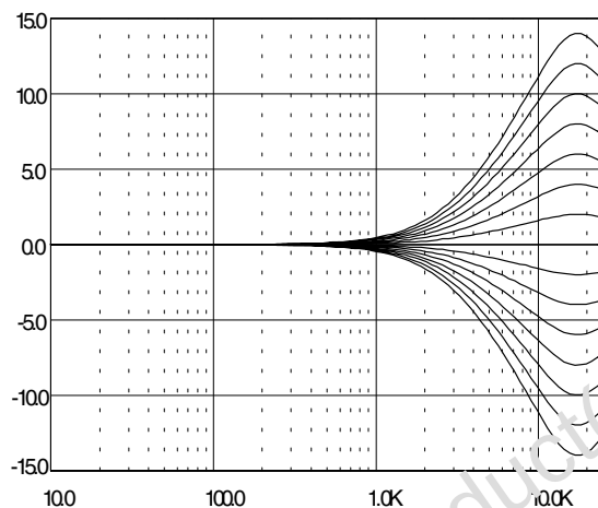
Figure 18. Treble Center Frequencies @ Gain = 14dB
