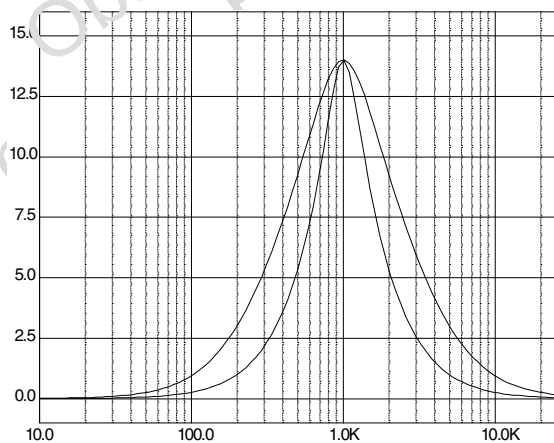
Figure 16. Mid Q-factor @ f_c=1\text{kHz} , Gain=14dB
