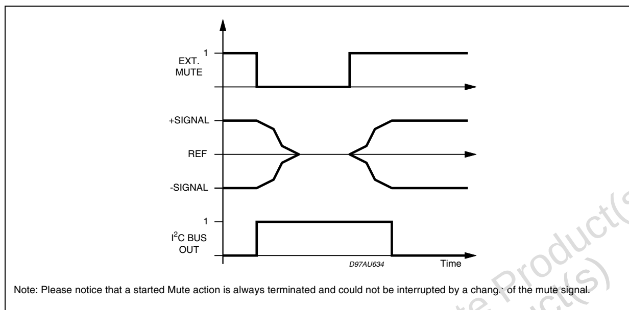
Figure 9. Softmute Timing
