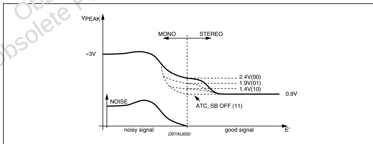
Figure 7. Fieldstrength Controlled Trigger Adjustment
