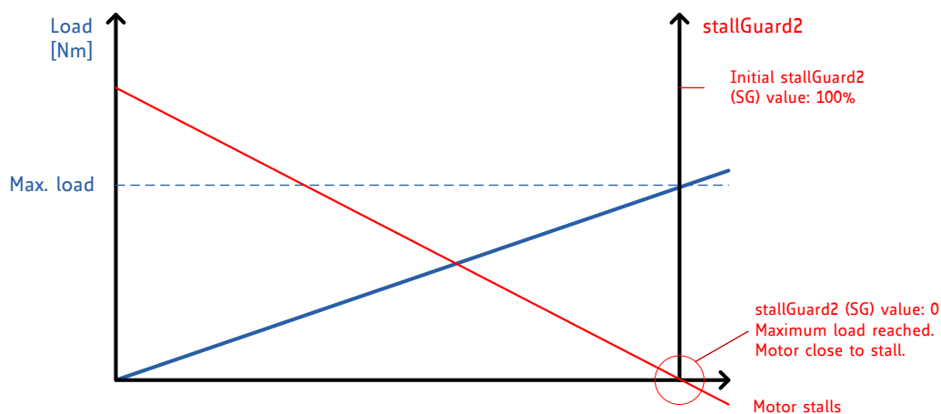
Figure 2.1 stallGuard2 load measurement SG as a function of load
