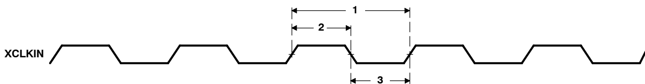
Figure 16. XCLKIN Timings
