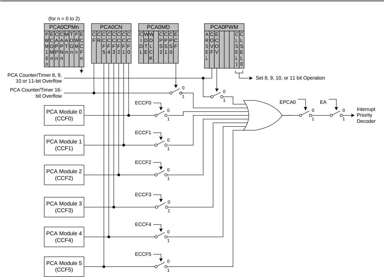
Figure 24.3. PCA Interrupt Block Diagram
