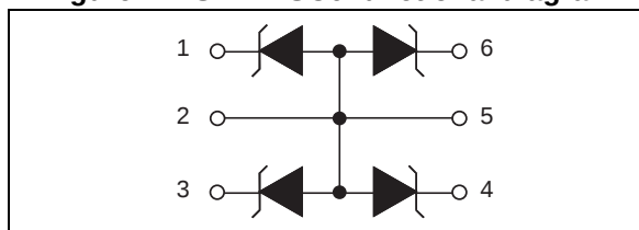
Figure 2. ESDAxxSC6 functional diagram
