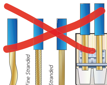
Not to be used with stranded or fine-stranded conductors
