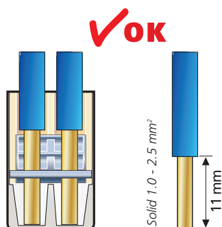
Solid conductors must be inserted completely
