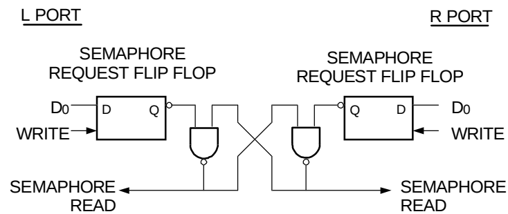
Figure 4. IDT7005 Semaphore Logic
