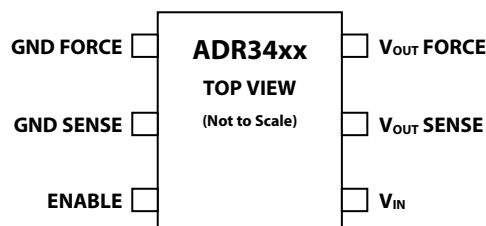
Figure 1. 6-Lead SOT23
