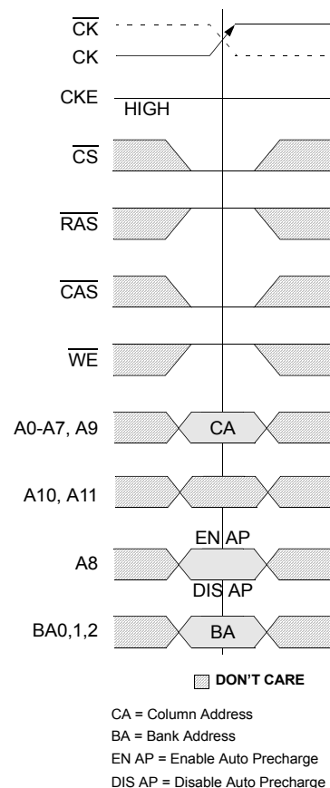
READ Command
