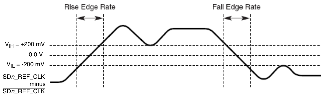
Figure 47. Differential Measurement Points for Rise and Fall Time
