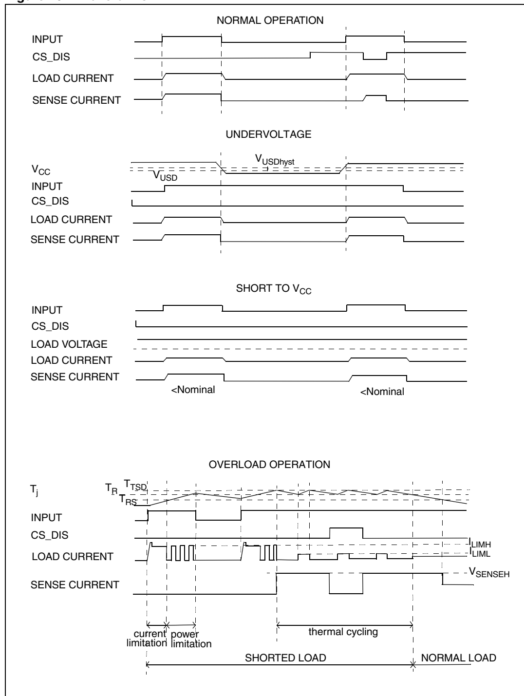
Figure 10. Waveforms
