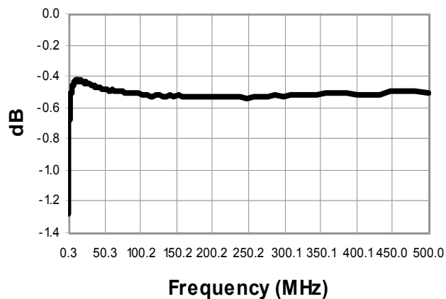
Amplitude Unbalance
