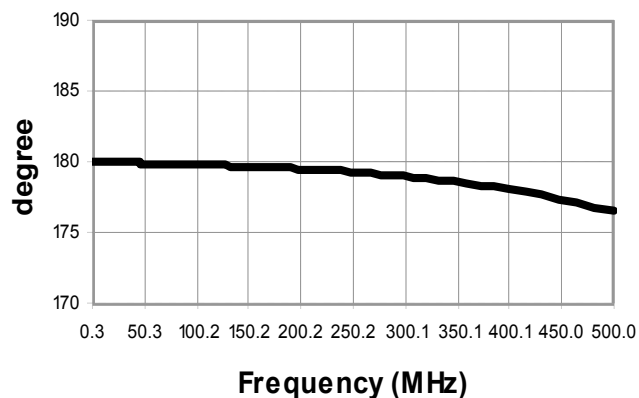
Phase Unbalance
