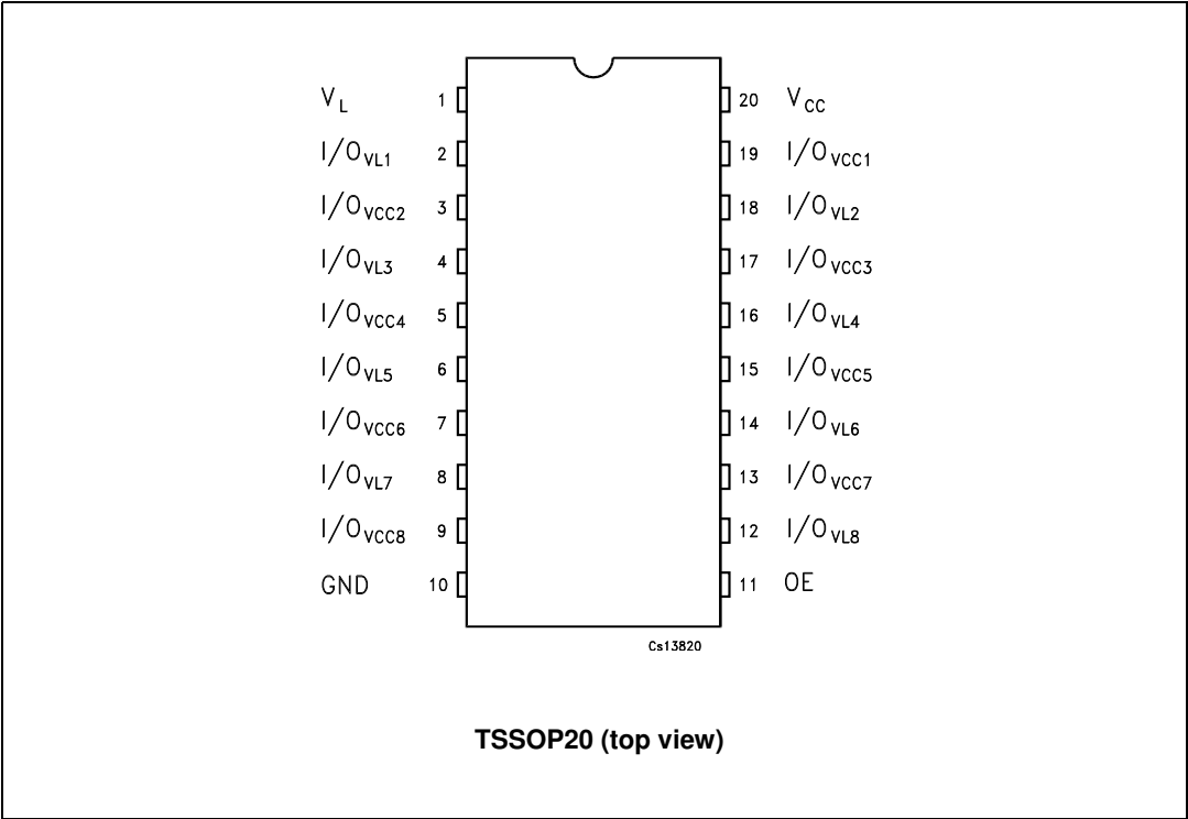
Figure 3. Pin connection
