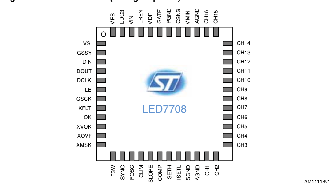
Figure 2. Pin connection (through top view)
