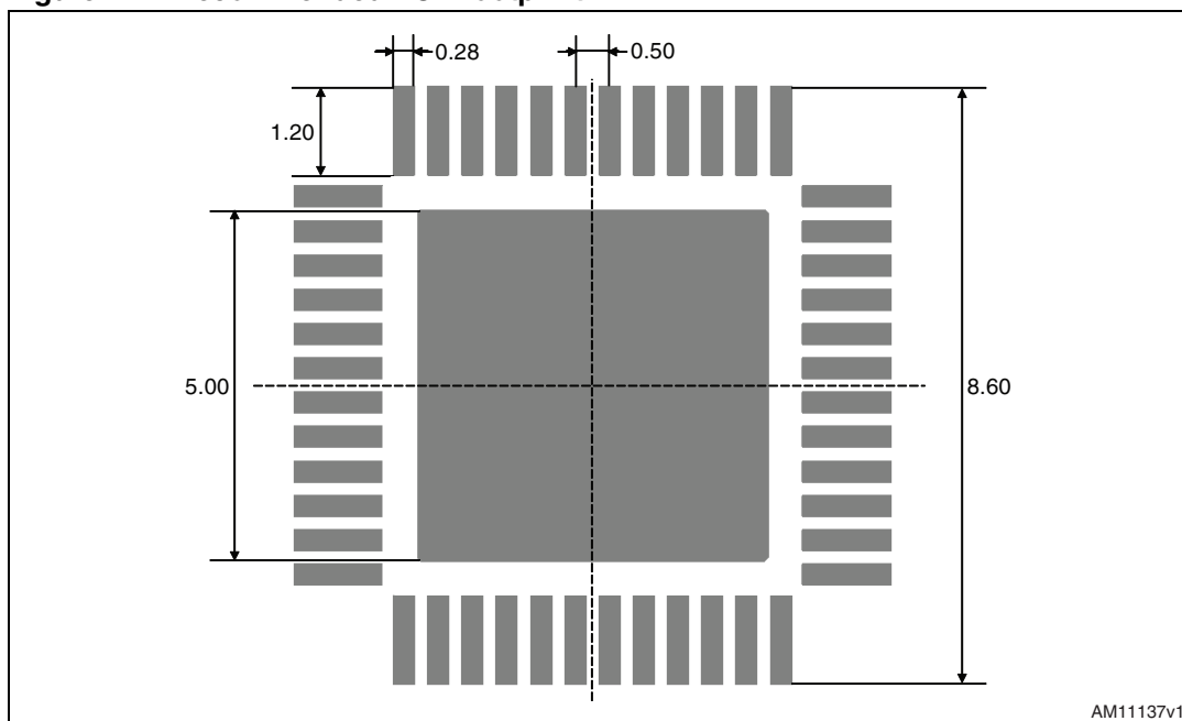
Figure 22. Recommended PCB footprint
