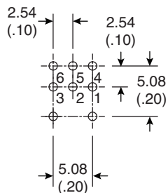
P.C. Mounting
