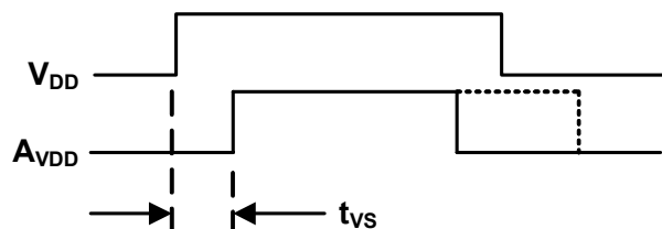
FIGURE 6. POWER SUPPLY SEQUENCE
