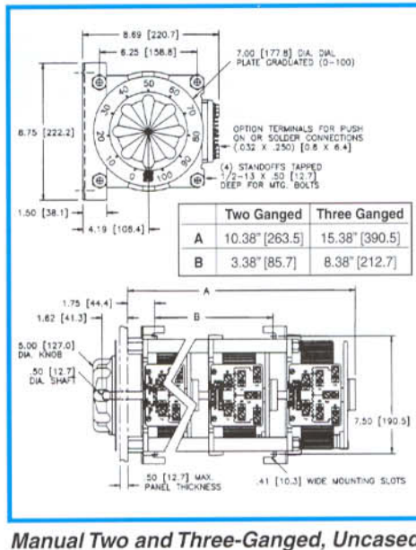
Manual Two and Three-Ganged, Uncased
