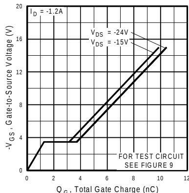
Fig 20. Typical Gate Charge Vs. Gate-to-Source Voltage
