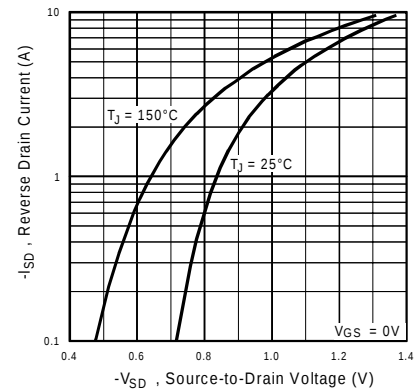
Fig 14. Typical Source-Drain Diode Forward Voltage
