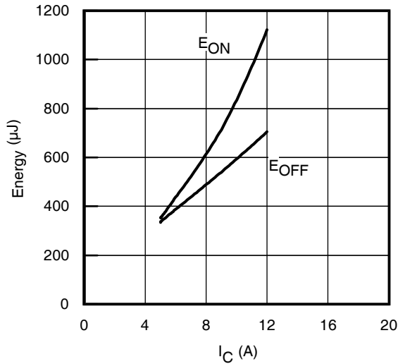
Fig. 13 - Typ. Energy Loss vs. I_C T_J = 125^\circ C ; L = 3.7mH ; V_{CE} = 600V R_G = 50\Omega ; V_{GE} = 15V
