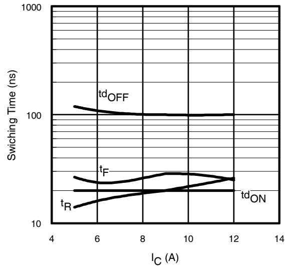
Fig. 14 - Typ. Switching Time vs. I_C T_J = 125^\circ C ; L = 3.7mH ; V_{CE} = 600V R_G = 50\Omega ; V_{GE} = 15V
