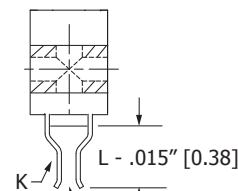
CARD EXTENDER REQUIRES -S288 MODIFICATION CODE (CS,CM,CT,RS,CK,TK,RM)
