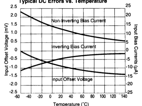
Typical DC Errors vs. Temperature
