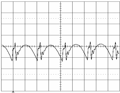
Output voltage ripple (20mV/div) at: T_{ref} = +25^{\circ}\text{C} , I_O = 6\text{ A} resistive load, V_I = 12\text{ V} . Time scale: 2 μs/div See the filter in the Output ripple and noise section (EMC Specification).
