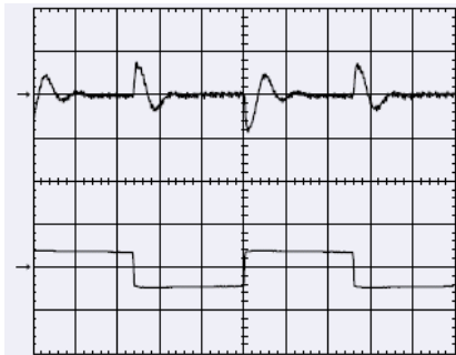
Output voltage response to load current step- change (-2A-2A) at: T_{ref} = +25^{\circ}\text{C} , V_I = 12\text{ V} . Top trace: V_{out} - V_{trk} (50mV/div). Bottom trace: load current (5 A/div). Time scale: 0.1 ms/div.
