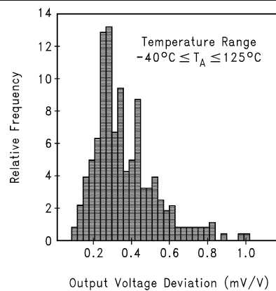
Figure 5-5. Thermal Hysteresis
