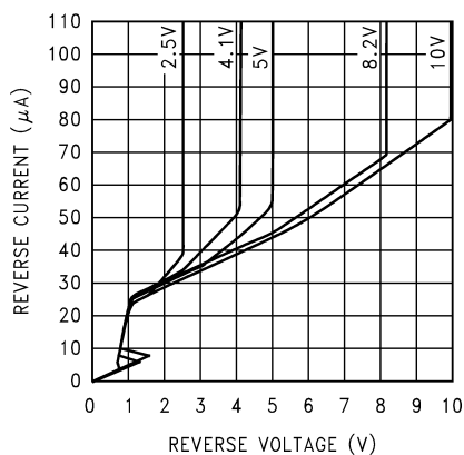
Figure 8-2. Reverse Characteristics and Minimum Operating Current
