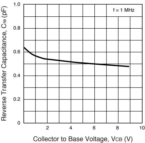
REVERSE TRANSFR CAPACITANCE vs. COLLECTOR TO BASE VOLTAGE
