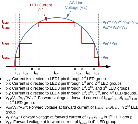
Figure 10. FL77904 Operation
