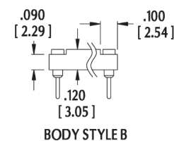
BODY STYLE B
