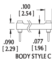
BODY STYLE C
