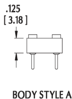
BODY STYLE A
