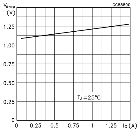
Figure 10. Dropout voltage vs. output current
