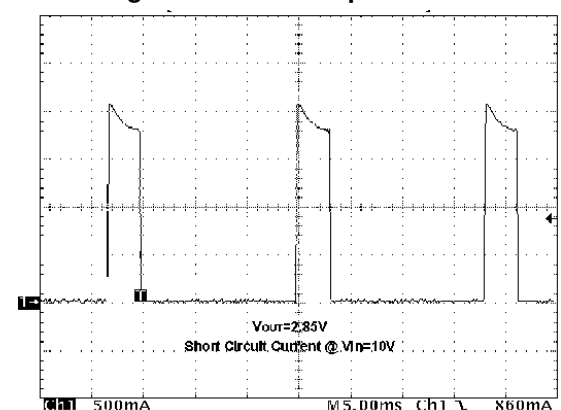
Figure 27. Thermal protection
