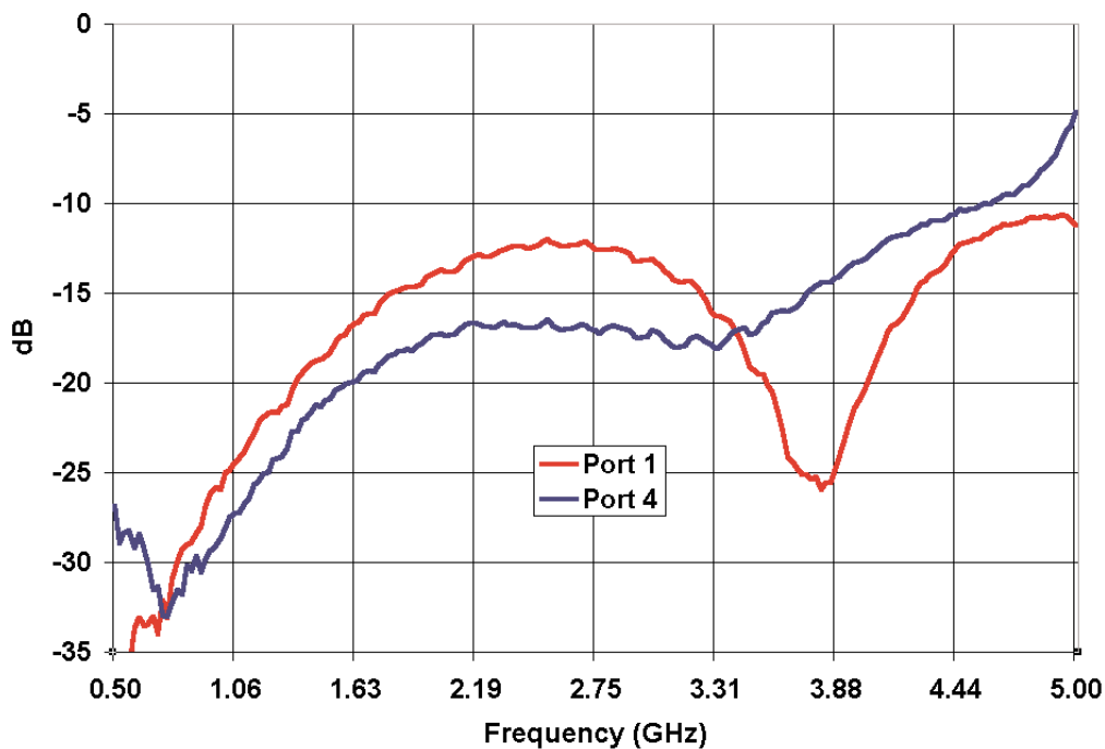
P/N 1748CP15A075 Coupler Typical Return Loss
