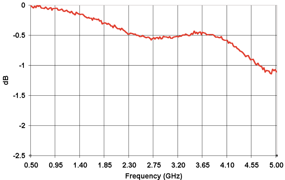
P/N 1748CP15A075 Coupler Typical Insertion Loss
