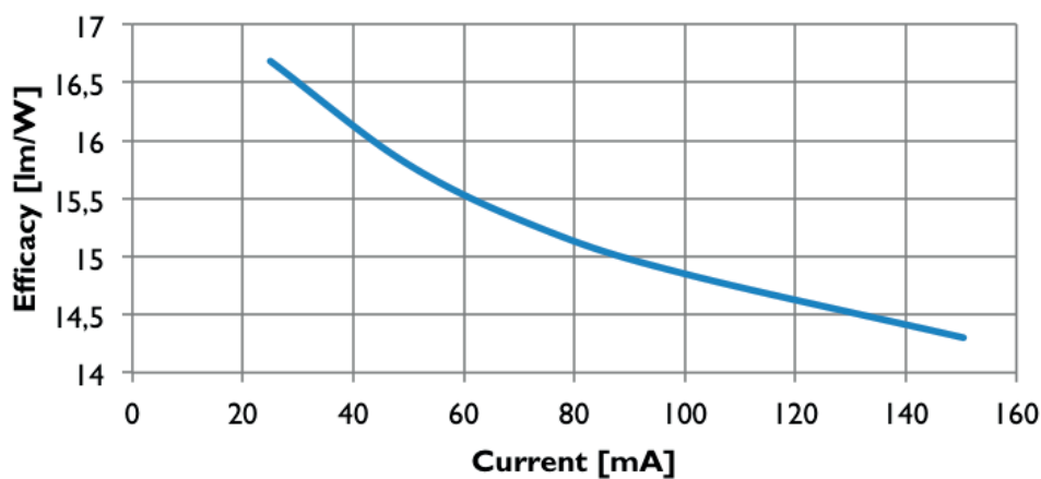
Luminous efficacy
