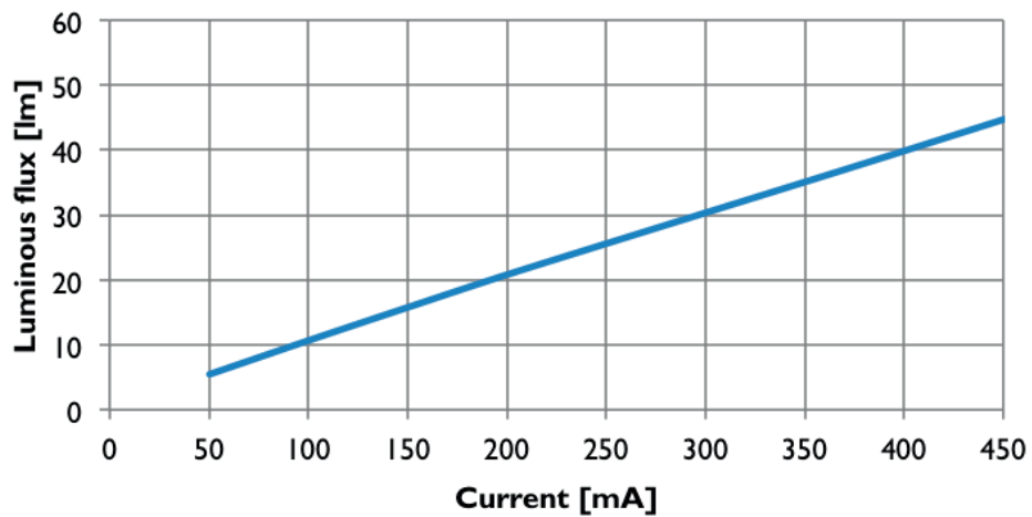
Luminous flux
