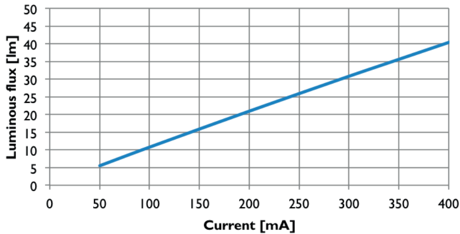
Luminous flux
