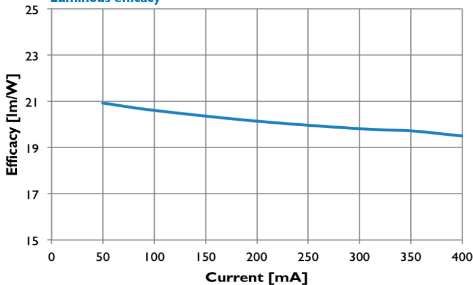
Luminous efficacy
