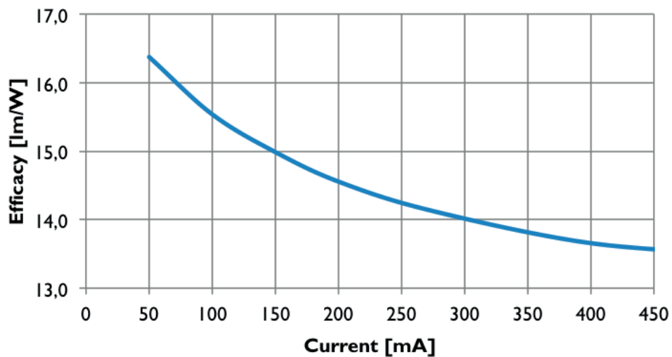
Luminous efficacy
