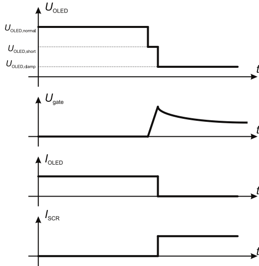
Figure 8: Idealized typical waveforms of the separate failure detection circuit.
