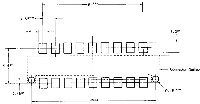
PC Board Layout (Connectors mount side)
