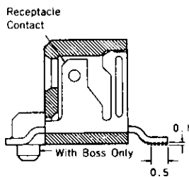
Section X-X
